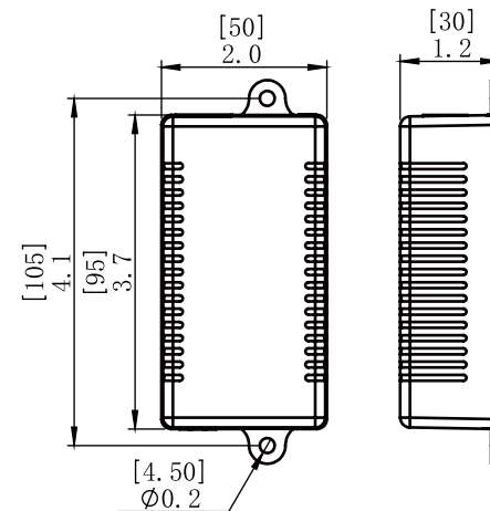
(sensor power)
