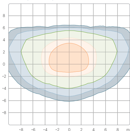
300W / 5000K / TYPE III
