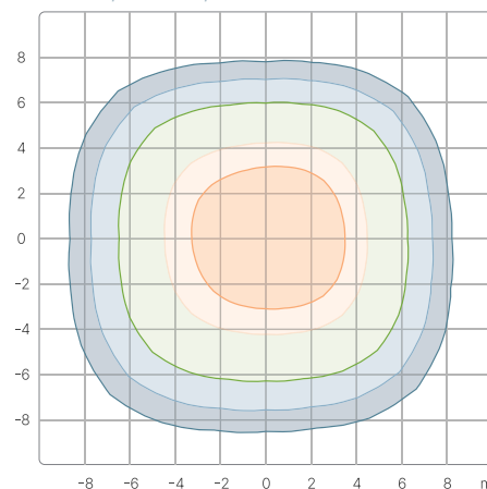
300W / 5000K / TYPE V
