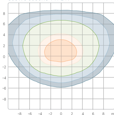
300W / 5000K / TYPE IV
