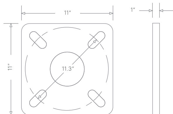
5" ANCHOR BASE
