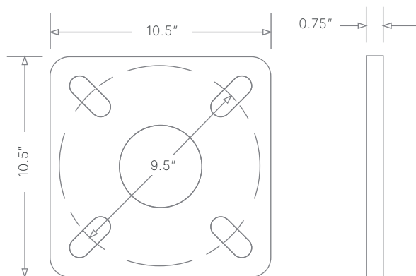
4" ANCHOR BASE
