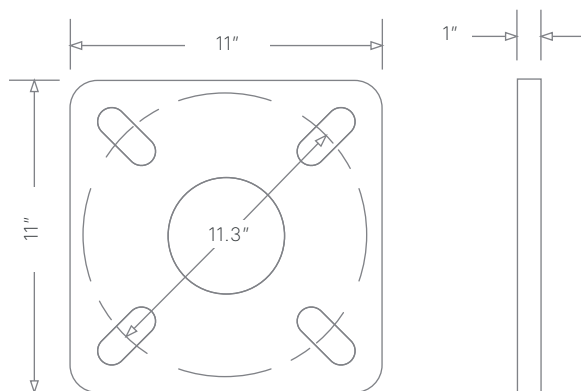
5" ANCHOR BASE
