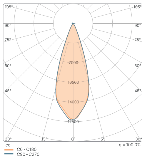
8" / 58W / 3000K / WIDE 36°
