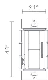
WITHOUT COVERPLATE
