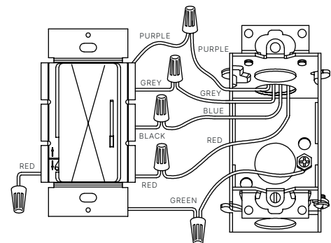
ON/OFF CONTROL WALLBOX WIRING
