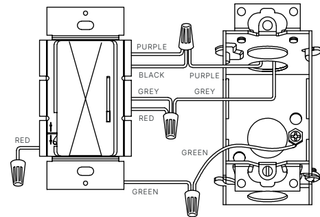
DIMMING ONLY WALLBOX WIRING
