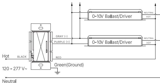
SINGLE POLE WIRING
