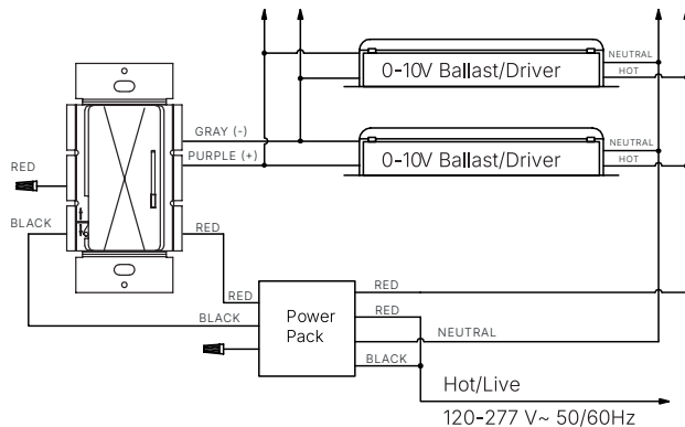
ON/OFF CONTROL W/ POWERPACK
