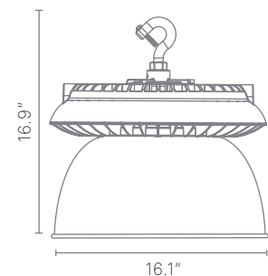
PC REFLECTOR
