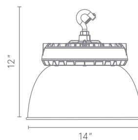
ALUMINUM REFLECTOR
